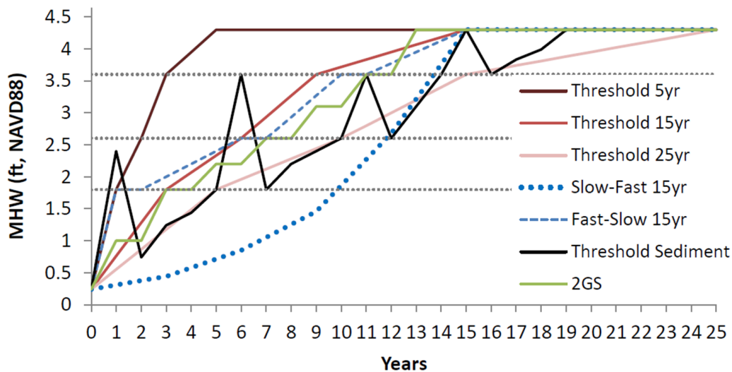
Figure 8B-1. Comparison of Predicted Mean High Water (MHW) Levels for the Full Herring River Restoration Project in the Lower Herring River Sub-basin Among Different Platform Policies. Maximum MHW elevations would not exceed 3.6 feet (NAVD88; top dotted line) for Phase 1 of the Project
