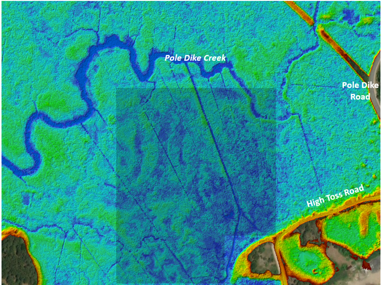
Figure 8B-2. Area North of High Toss Road Where Extensive Grid Ditching Has Led to Severe Subsidence of Marsh Surface (Shaded Area)
