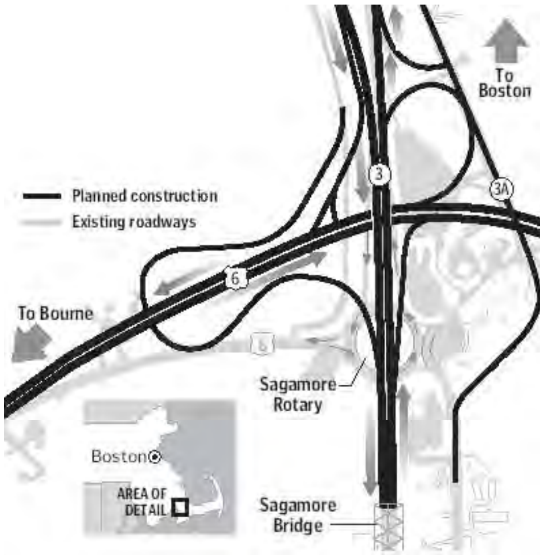
FIGURE 10 - SAGAMORE INTERCHANGE DIAGRAM
