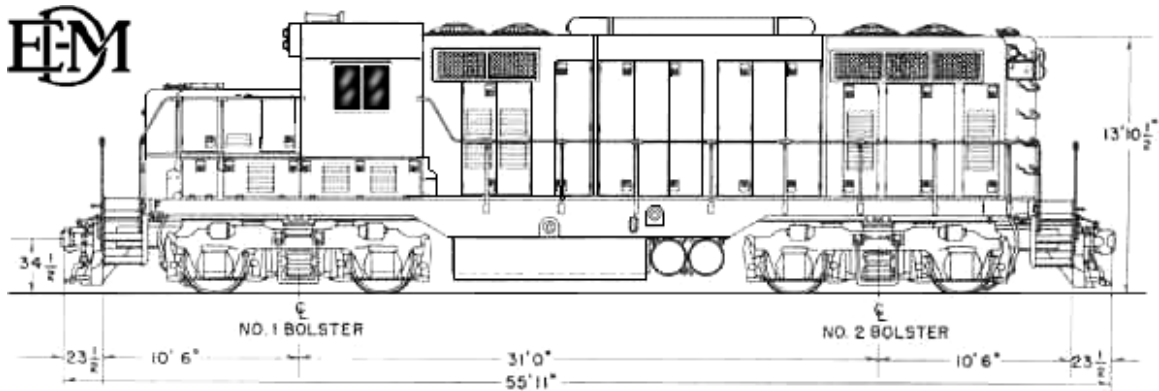
FIGURE 35: DIAGRAM FOR ENGINES 1501 AND 1502
