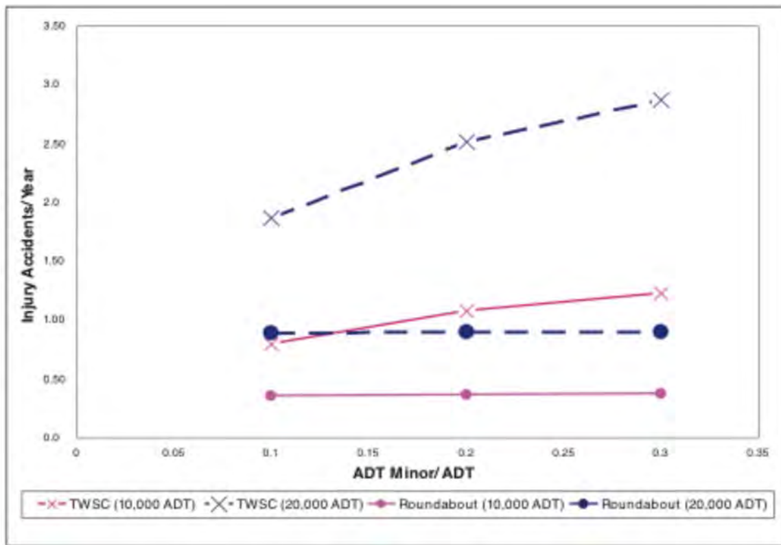
FIGURE 3 - COMPARISON OF PREDICTED ROUNDABOUT INJURY CRASHES WITH RURAL 2-WAY STOP -CONTROLLED INTERSECTIONS.
