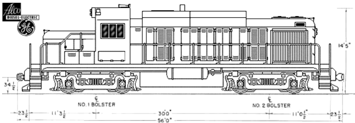
FIGURE 36: DIAGRAM FOR ENGINE 1201
