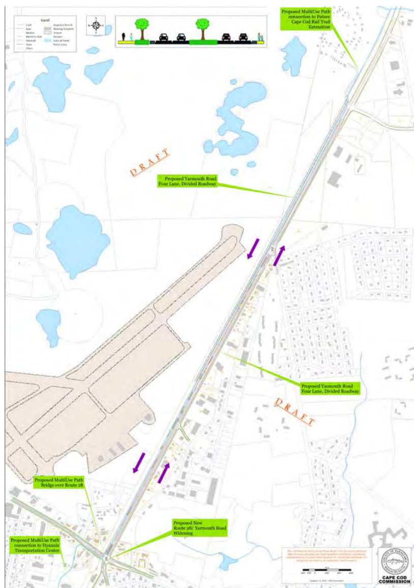
FIGURE 53 - YARMOUTH ROAD RECOMMENDED CONCEPT PLAN
