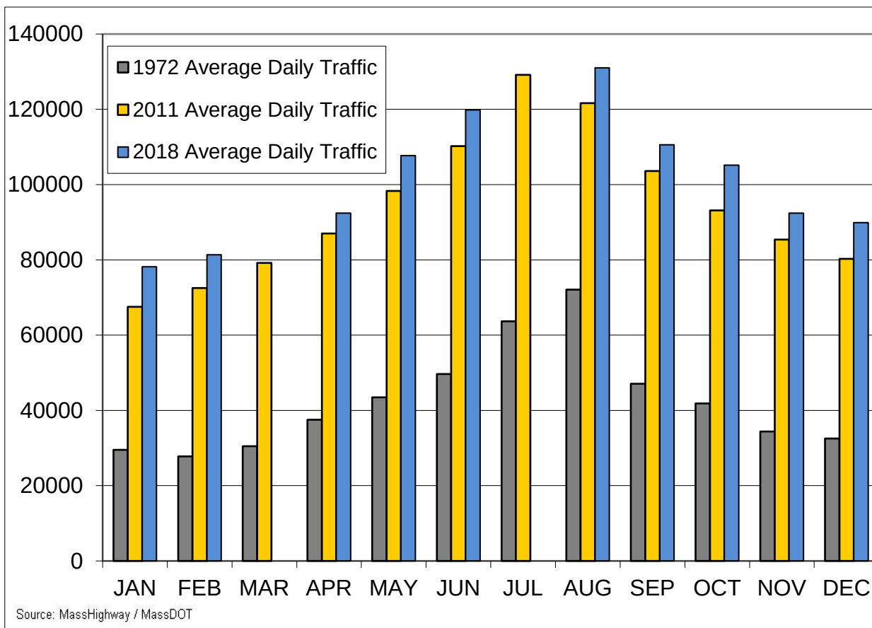
Figure 2: Historic Monthly ADT Changes at the Bourne and Sagamore Bridges
