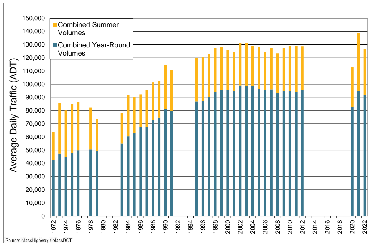
Figure 1: Combined Average Daily Traffic over Bourne and Sagamore Bridges
